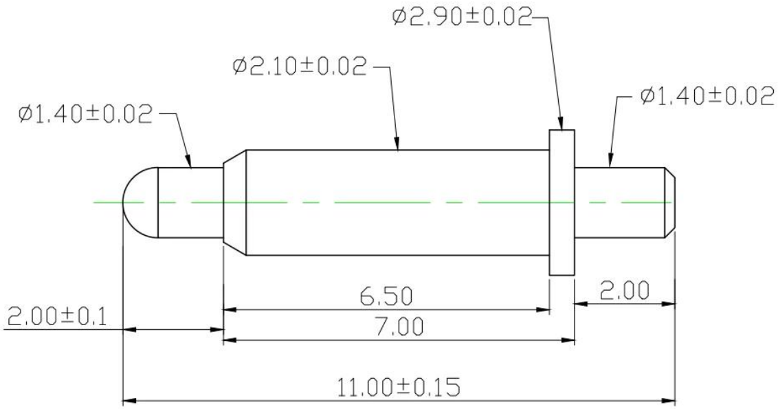
pogo pin drawing:
