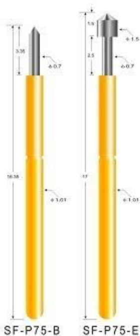
PCB test probe pin product photo
