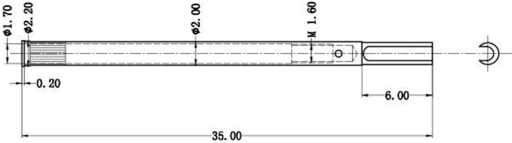
Cable Harness Test Probe with thread screw test equipment:
