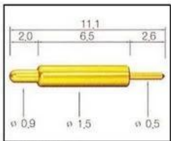
SF-P111G-150
