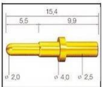
SF-P154G-250
