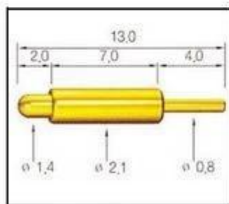
SF-P130G-210
