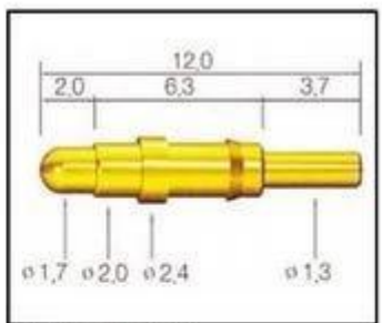
SF-P120G-200
