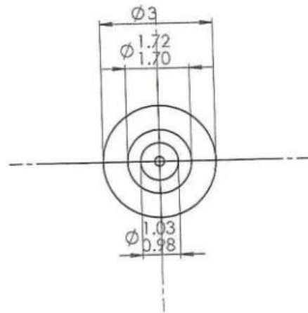
terminal pin: SF-Pin 3.0*6.9mm
