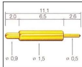
SF-P111G-150
