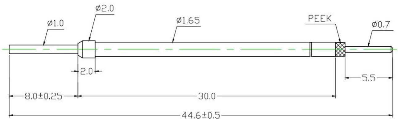
Switching test probe drawing
