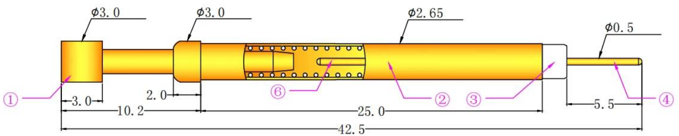
Switching test probe drawing
