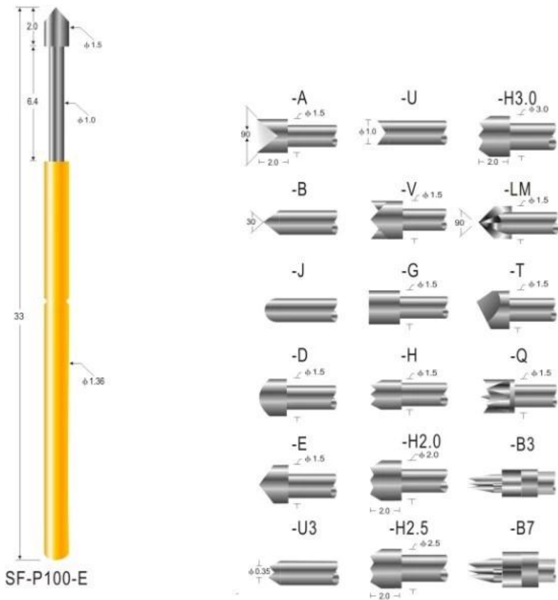
Spring loaded probe pin SF-P100 drawing
